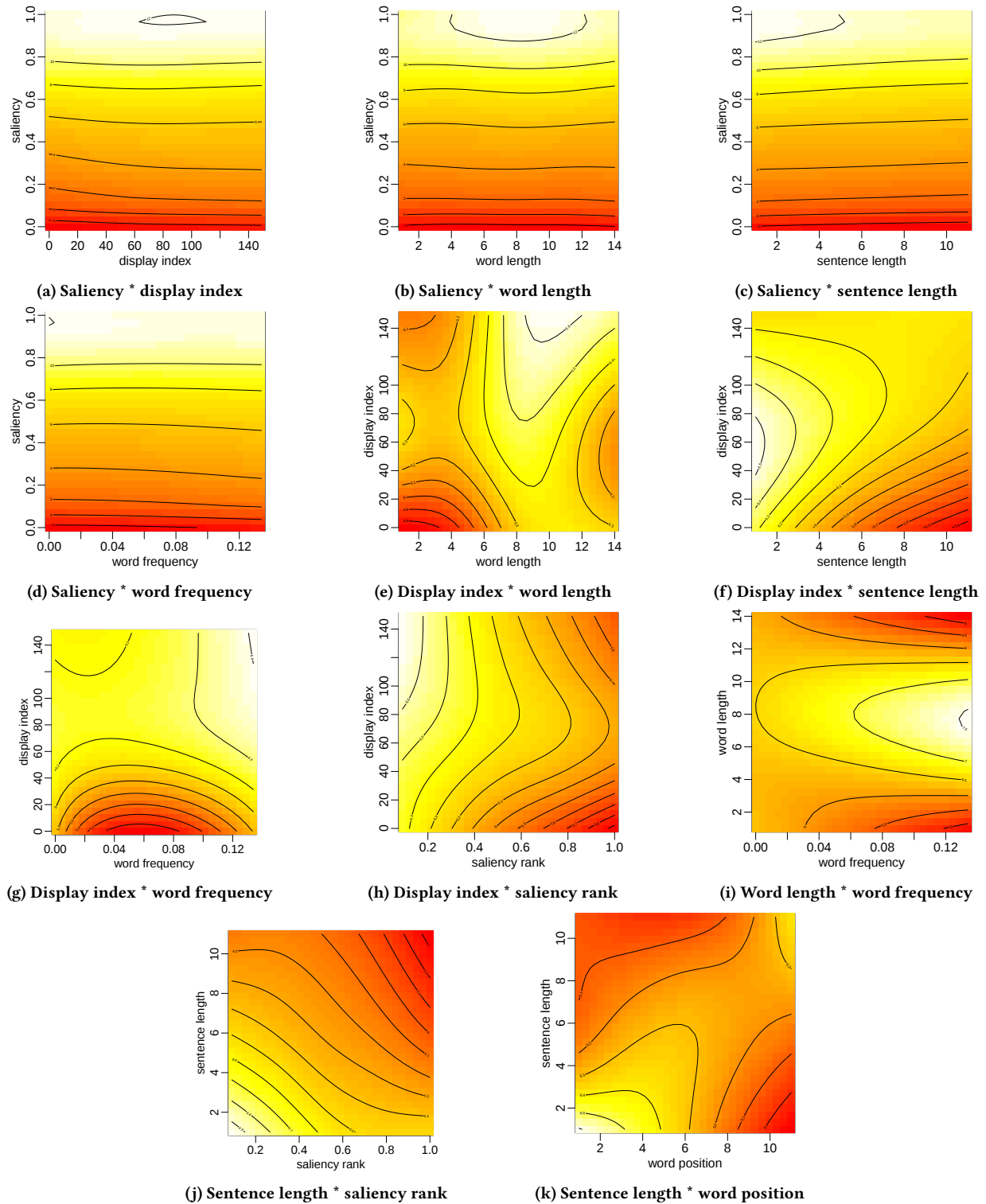
Figure 10: Summed effect plots of all significant pairwise interactions.
