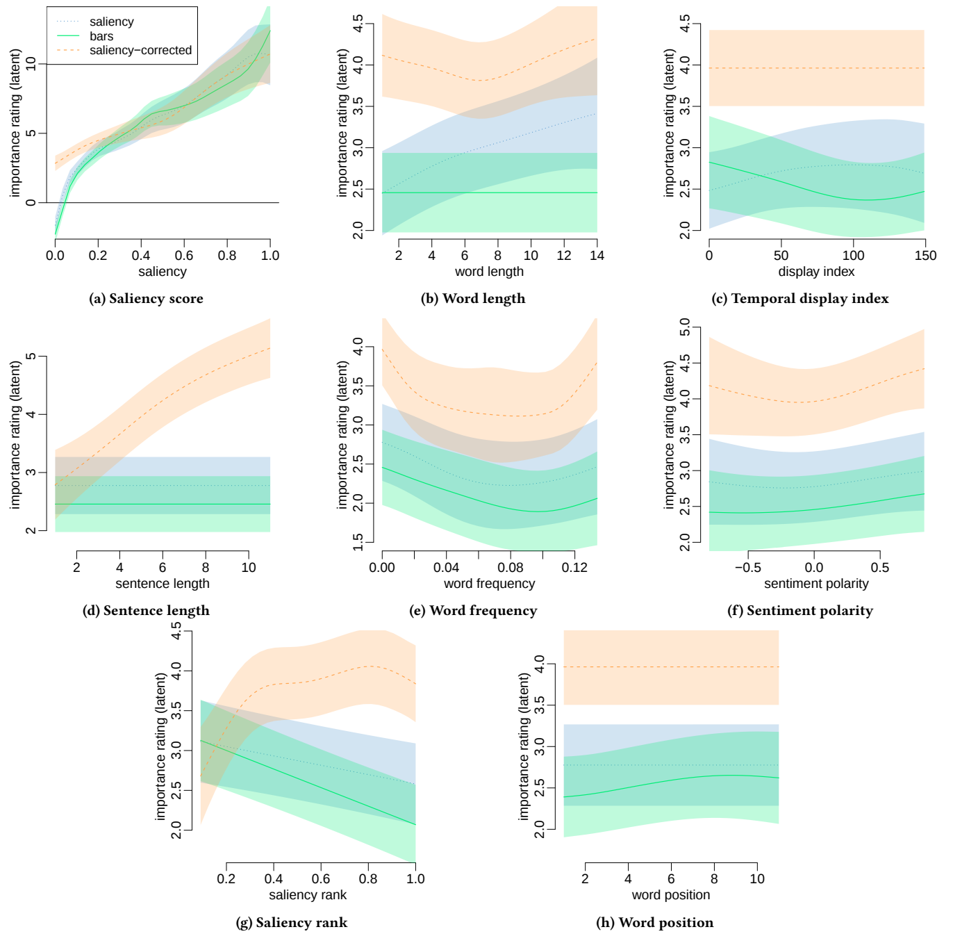
Figure 11: Summed-effects comparison plots of the correction methods.
