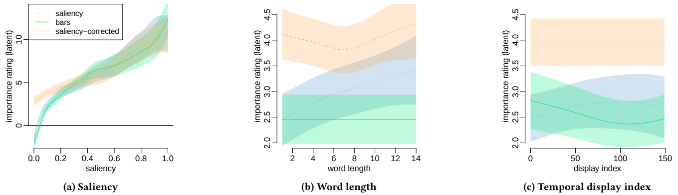
Figure 6: Selected summed-effects comparison plots of the visualization alternatives.
