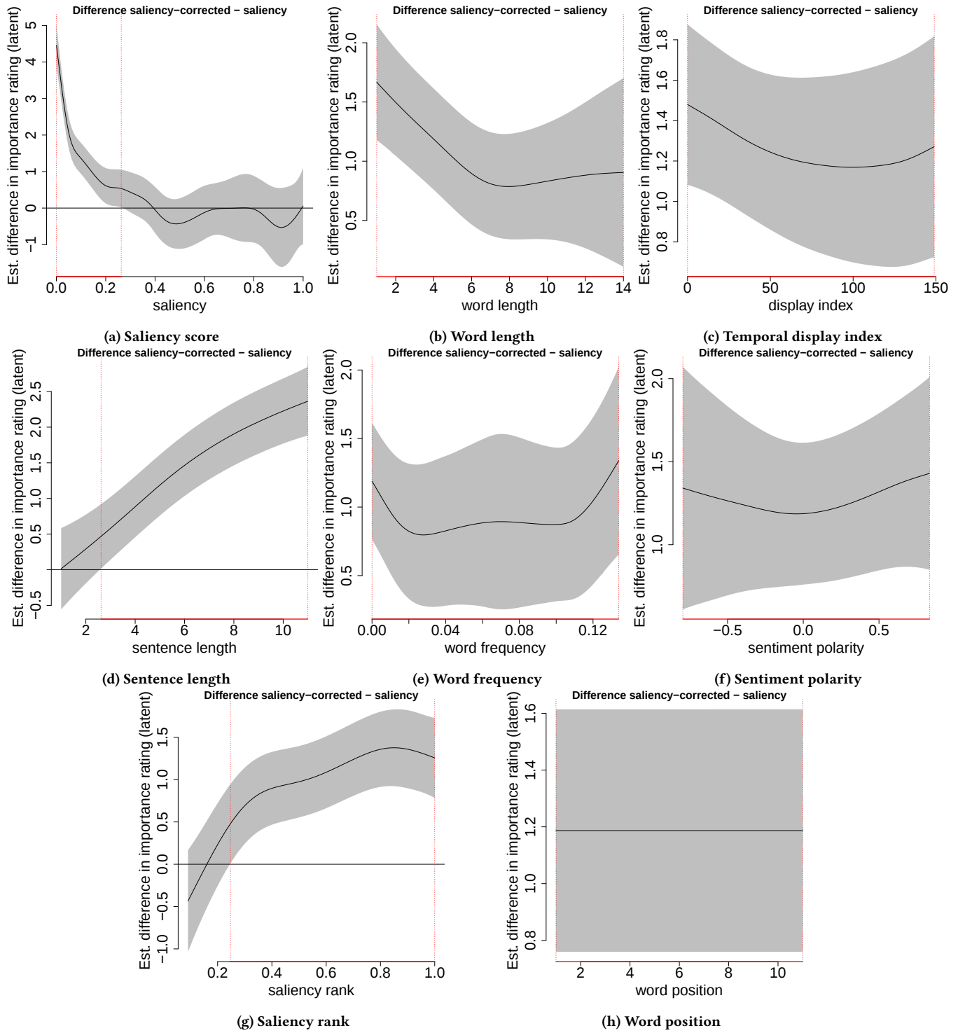
Figure 13: Difference plots between the model-corrected saliencies and original saliencies. Areas of significant differences are marked red.
