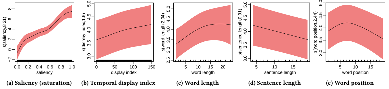
Figure 4: Partial effect plots for all significant smooth terms (note that y-axes are scaled per effect) for the German experiment. Numbers in y-axis labels are estimated degrees of freedom (edf) of the respective smooth. The shaded area displays confidence intervals (plus and minus one standard error) including uncertainty about the overall mean. (a) refers to color saturation.
