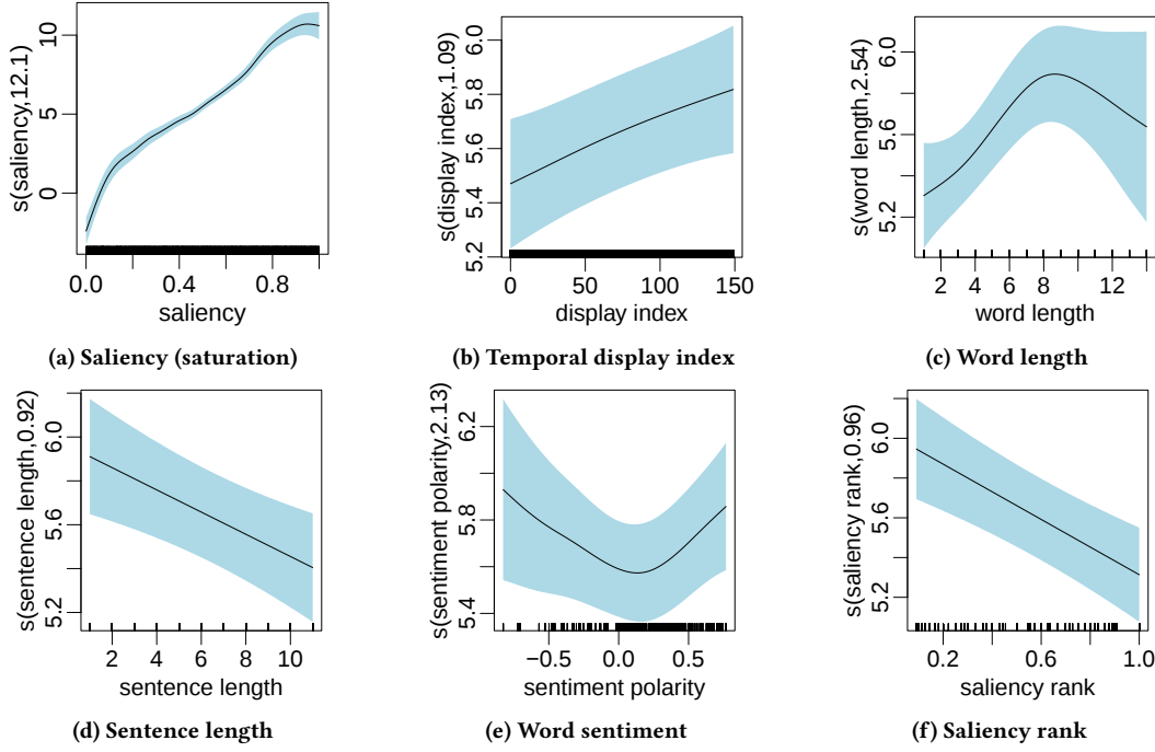
Figure 3: Partial effect plots for all significant smooth terms (note that y-axes are scaled per effect). Numbers in y-axis labels are estimated degrees of freedom (edf) of the respective smooth. The shaded area displays confidence intervals (plus and minus one standard error) including uncertainty about the overall mean.
