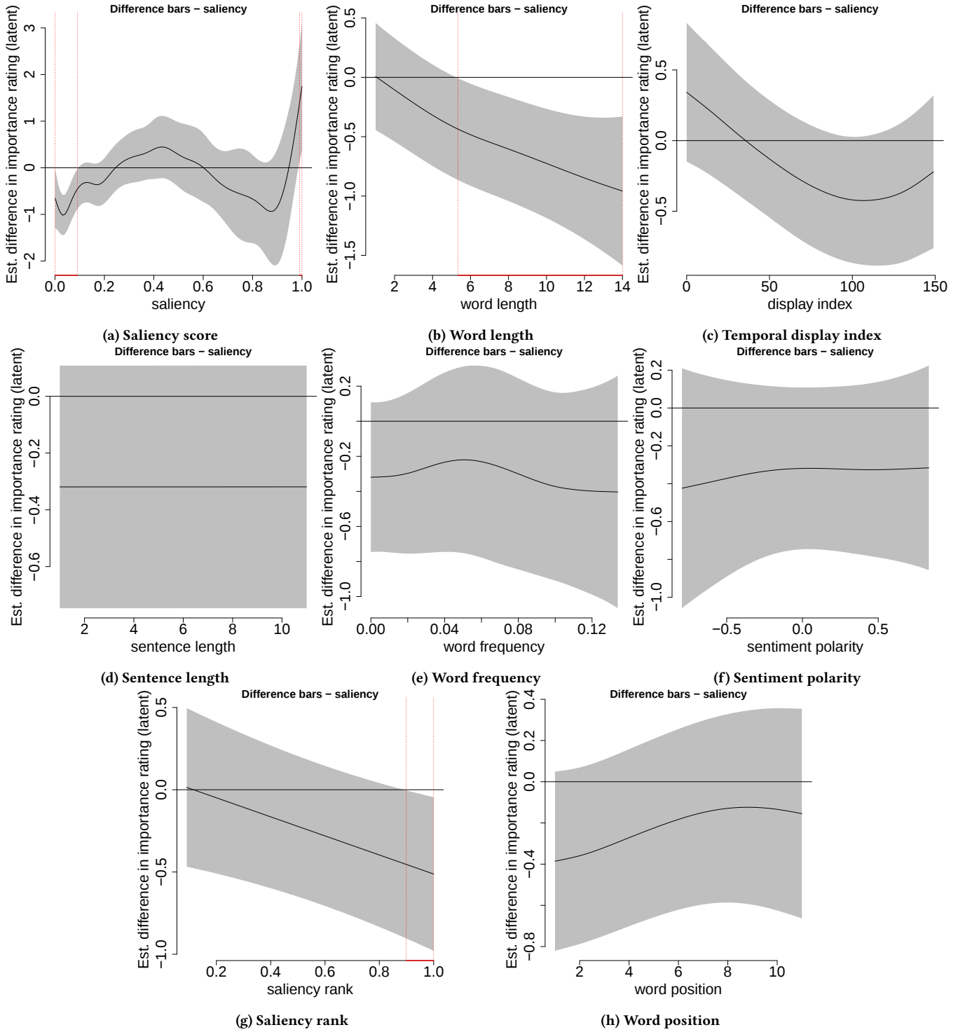
Figure 12: Difference plots between the bar visualization and the original visualization. Areas of significant differences are marked red.
