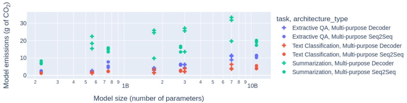
Figure 5: A plot of the total emissions (in grams of CO_2eq ) for 1,000 inferences for all multi-purpose models.
